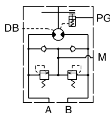
Hydraulic symbol (CHB type)
